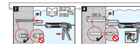
FIGURE 8A—MANUFACTURER'S PRINTED INSTALLATION INSTRUCTIONS (MPII) (Continued)
